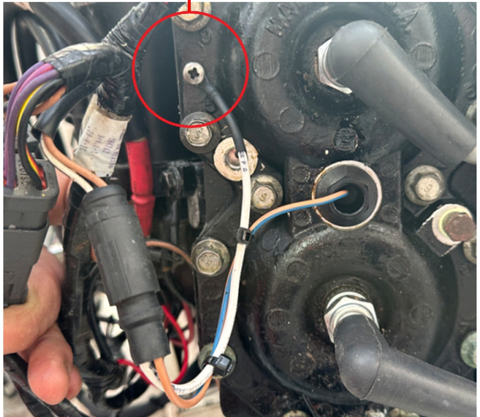
0585185 – Substitute Temp Switch (After Modification – Installed)
