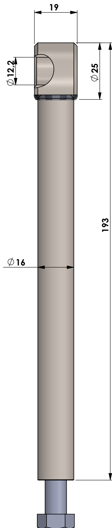
Cod.92386088141: stem eyelet for trim AQ290 DP-SP-DPX (original cod.3860881) mm/inch version.
