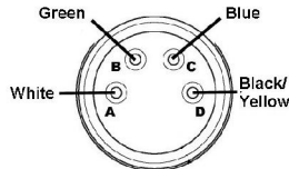
WIRE SIDE VIEW
